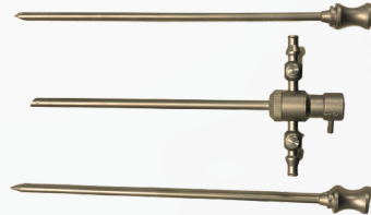
SHEATH WITH TROCAR
